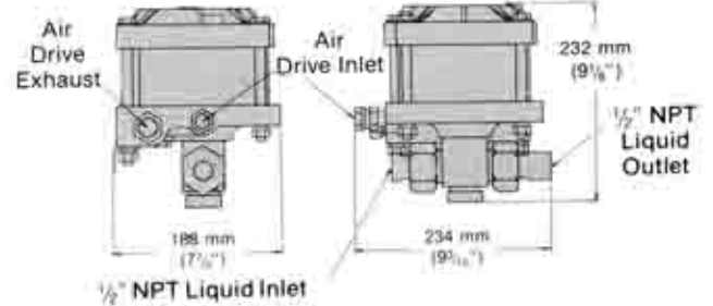
1.5 & 2 HP Medium & High Ratios -25 thru -150, -151, -225, -300 and -450 Ratios
