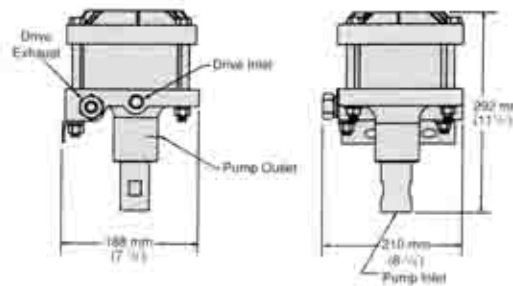
AFD or ASFD - B60 PUMP Double Acting – High Output
